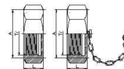
Hexagon Blind Nut(With Chain)
