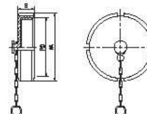
DIN blind nut with chain
