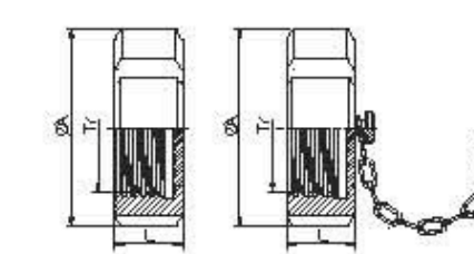
IDF-13 Blind Nut(With Chain)
