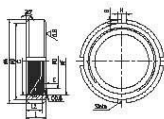
Round Nut
