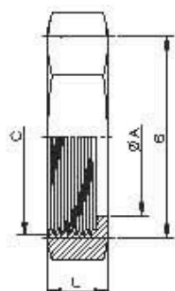
Hexagon Nut
