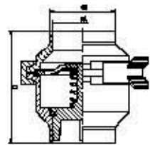
SMS check valve weld end
